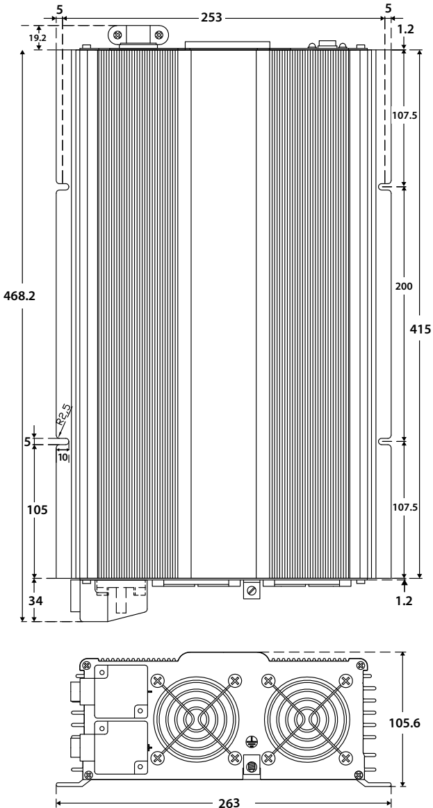
Fig. 8.1: PST-1500 and PST-2000 Overall Dimensions & Mounting Slots (NOTE: Dimensions in mm)
